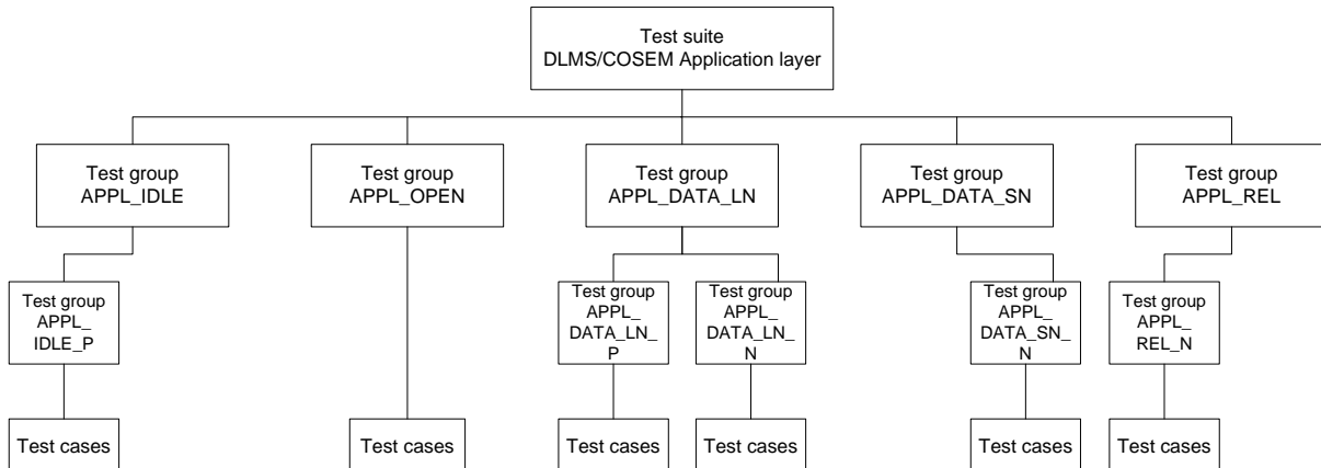
Figure 5 – Structure of the conformance test plan for the COSEM Application layer
